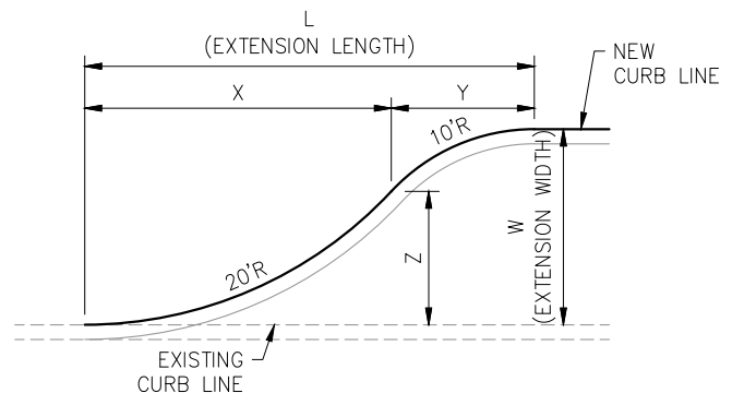
CURB EXTENSION DIMENSIONS
