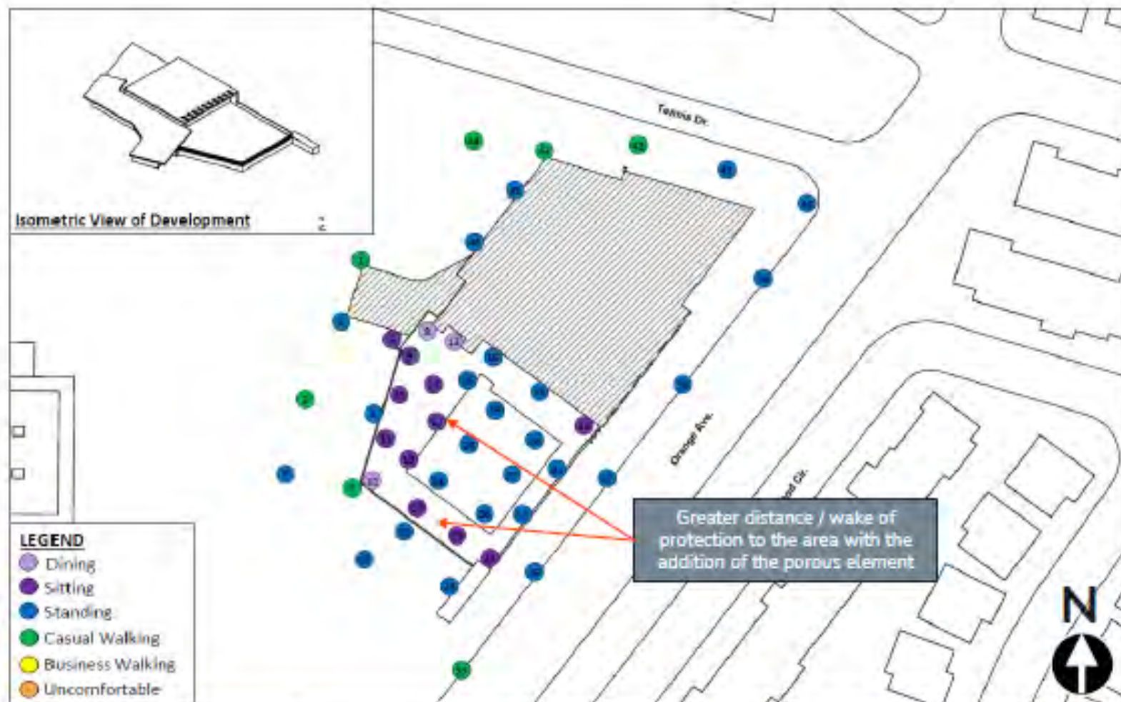
Pedestrian Wind Comfort Conditions – Operating Hours (January to December, 6:00am – 9:00pm)
